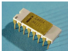
Gambar 2.23 Chip Intel 4004
