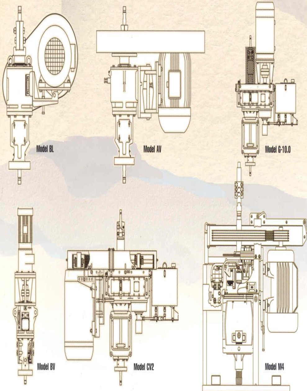
Gambar Tipe Drive Head
