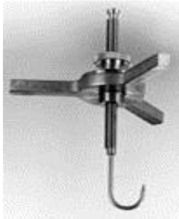
Gambar 160. Hook Gauge
