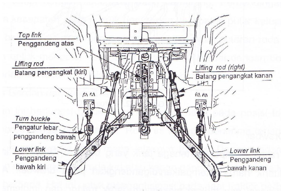
Gambar 120. Three point hitch
