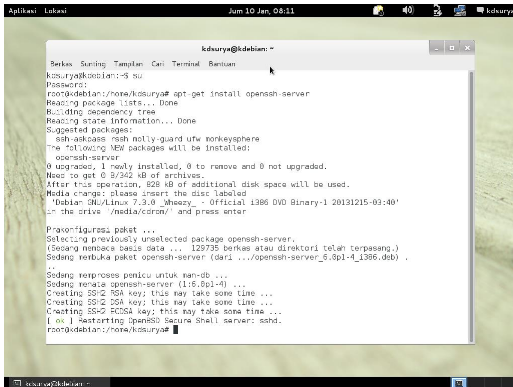
Gambar 38. Instalasi OpenSSH Server
