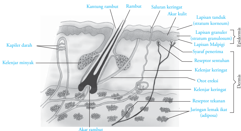
Gambar 8.5 Bagian-bagian kulit
