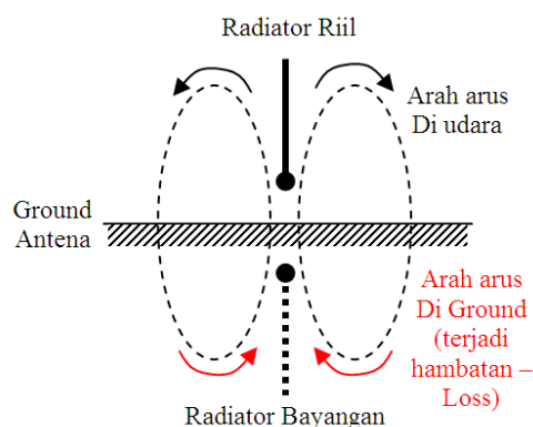
Gambar 7.11. Ground Loss
