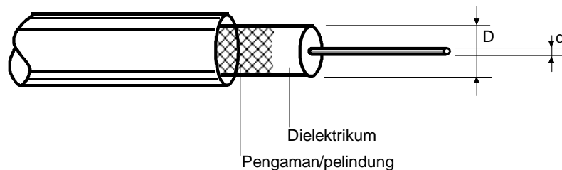
Gambar 5.12. Penampang kabel Coaxial
