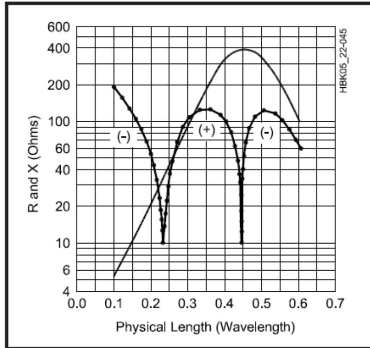
Gambar 7.14. Radiator length
