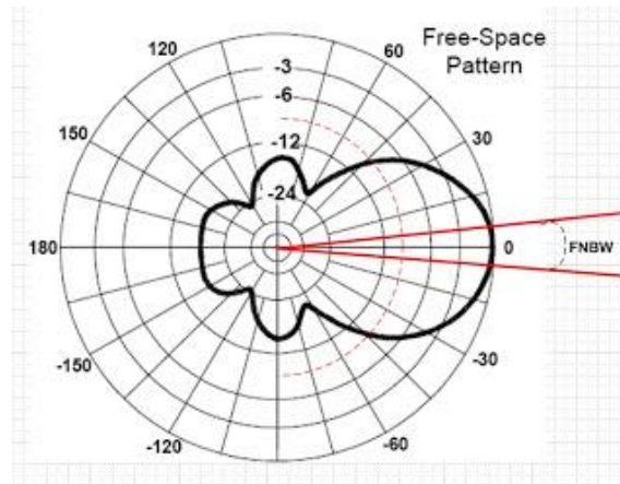
Gambar 4.5. First Null Beam Width
