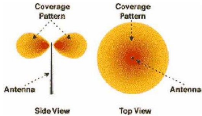
Gambar 6.5. Pola Radiasi Antena Omnidirectional
