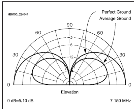
Gambar 7.12. Radiation pattern
