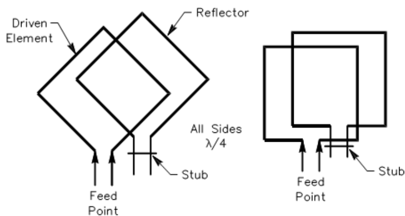
Gambar 10.1. Model antenna Quad Loop
