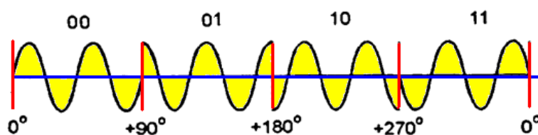
Gambar 4.31. Differential PSK
