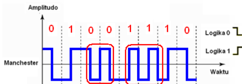
Gambar 1.9. Diagram pulsa pengkodean Manchester
