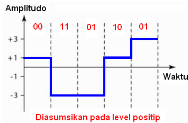
Gambar 1.13. Diagram pulsa pengkodean 2B1Q
