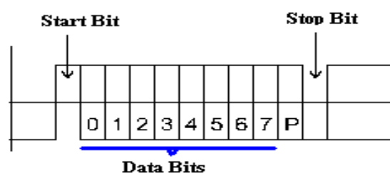
Gambar 4.17. Frame data protokol RS-232
