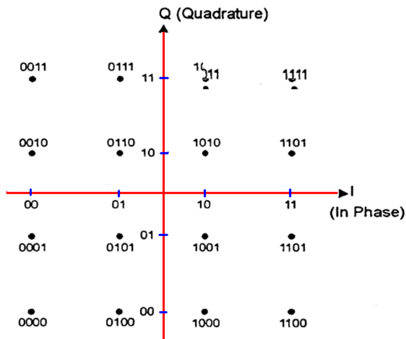
Gambar 4.32. CCITT V.22bis Quadrature Amplitude Modulation
